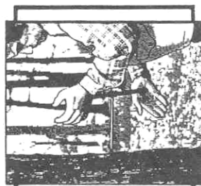
An Increment borer being used on a Southern yellow pine.
